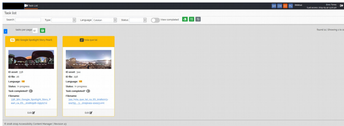
Figure 1: Editor interface
